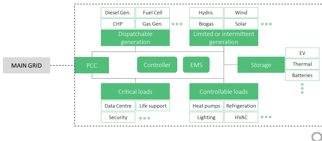
Figure 2 - General representation of a grid-connected microgrid 11
