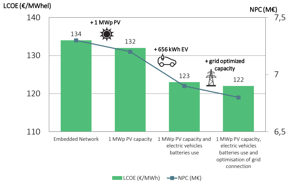
Figure 10 - Costs savings drivers for the airport as a smart embedded network (excluding networks costs)
