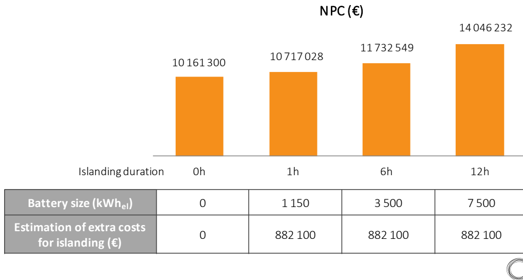
Figure 11 - Microgrid islanding (excluding networks costs)
