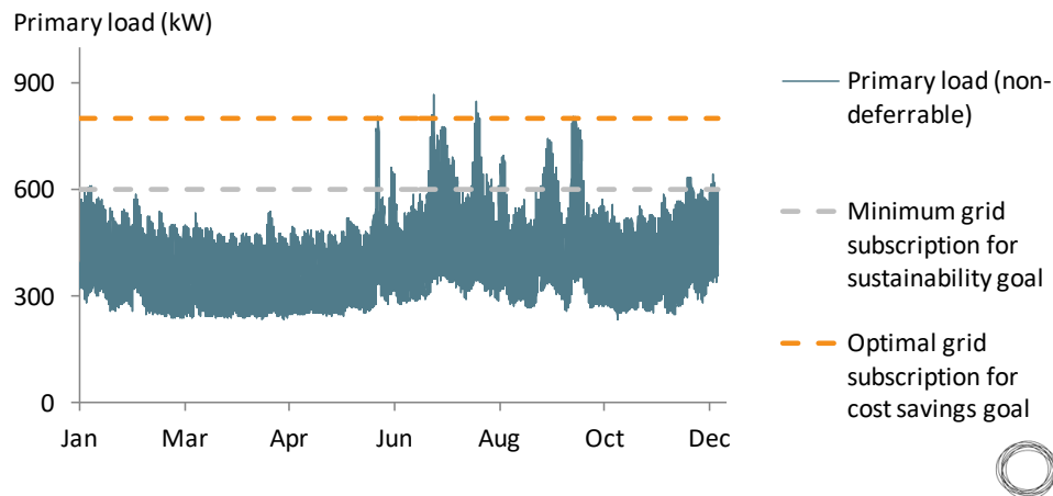
Figure 8 – Relevant grid subscription choices with respect to non-deferrable load profile
