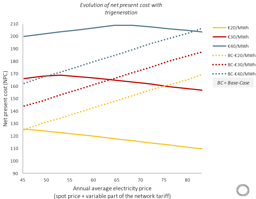
Figure 13 – Trigeneration case: Evolution of NPC with electricity and gas prices (excluding network costs)
