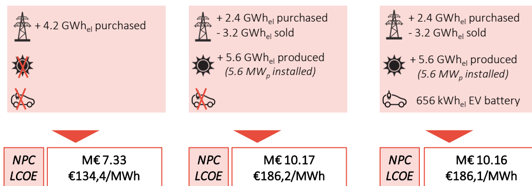
Figure 9 - Comparison of grid-only scenario with local generation scenarios (local generation only, use of vehicle-to-grid system, and use of a grid-scale battery) 23
