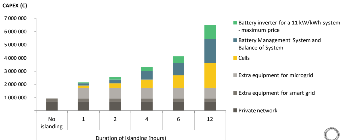
Figure 21 – CAPEX of equipment needed for the islanding function 50 depending on the required islanding time (Enea Consulting analysis based on [32, 33, 19, 34, 35, 36, 37] for grid equipment and [38, 39, 40, 41, 42] for batteries)
