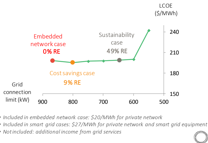
Figure 7 – Results of sensitivity analysis on maximum power delivered by the grid
